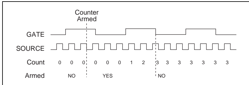
Figure 3-19. Frequency Measurement
