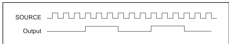
Figure 3-22. Frequency Division
