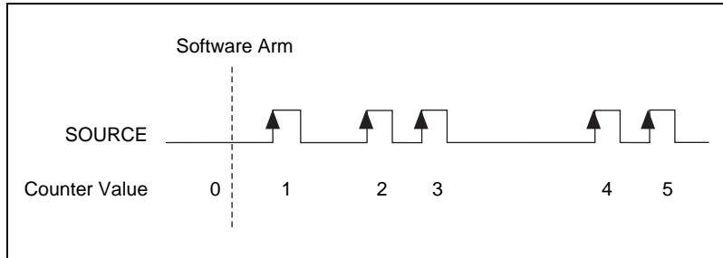
Figure 3-1. Simple Event Counting
