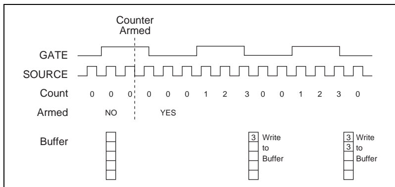
Figure 3-20. Buffered Frequency Measurement
