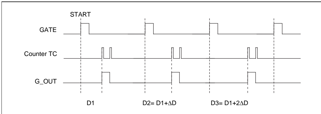
Figure 3-17. Pulse Generation for ETS
