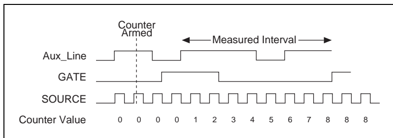
Figure 3-5. Two-Signal Edge-Separation Measurement
