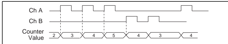
Figure 3-28. Two-Pulse Encoders
