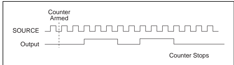
Figure 3-21. Finite Pulse-Train Generation
