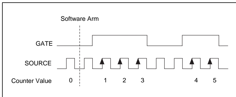
Figure 3-2. Gated-Event Counting
