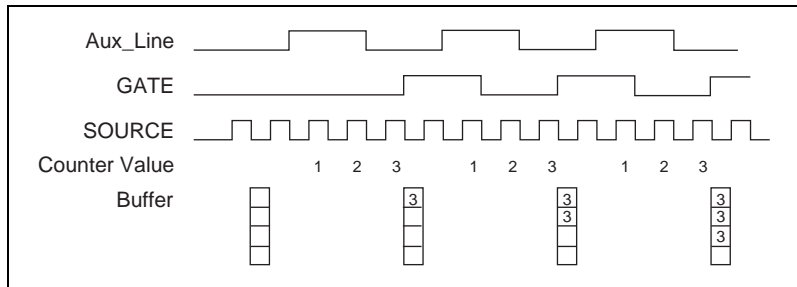
Figure 3-16. Buffered Two-Signal Edge-Separation Measurement
