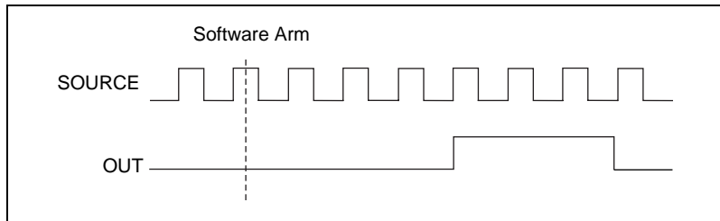
Figure 3-7. Single Pulse Generation
