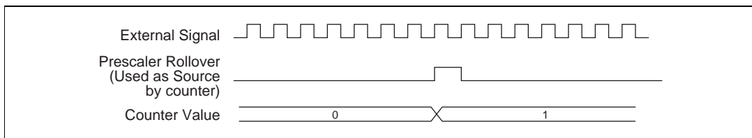
Figure 3-32. Prescaling
