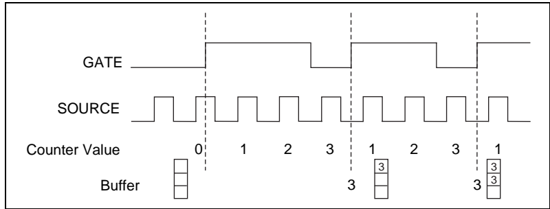
Figure 3-13. Buffered Period Measurement
