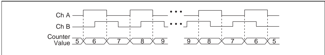
Figure 3-25. Position Measurement for X2 Encoders
