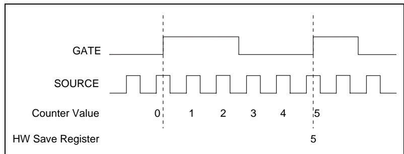
Figure 3-3. Single-Period Measurement
