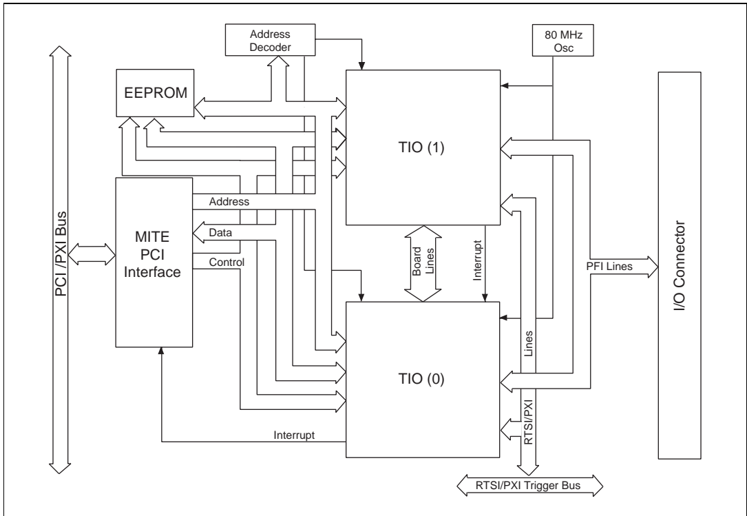
Figure C-1. PCI/PXI-6602 Block Diagram
