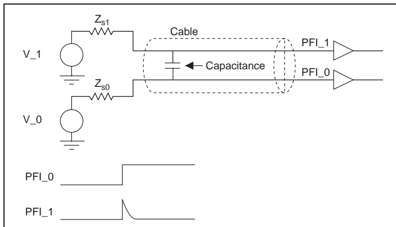
Figure 4-7. Crosstalk
