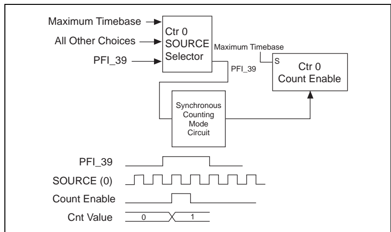
Figure 3-36. With Synchronous Counting Mode
