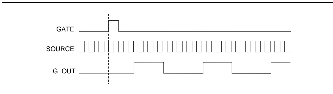
Figure 3-10. Continuous Pulse-Train Generation
