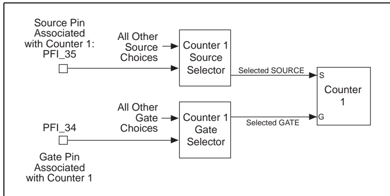
Figure 4-5. Counter Input
