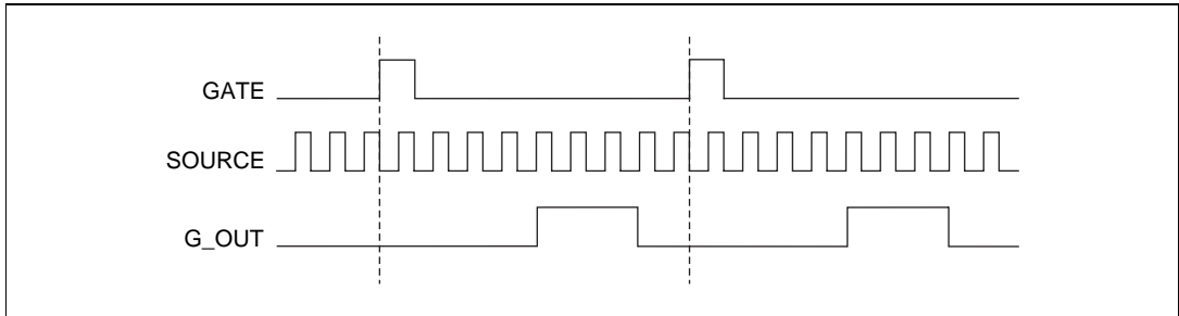
Figure 3-9. Retriggerable Single Pulse Generation
