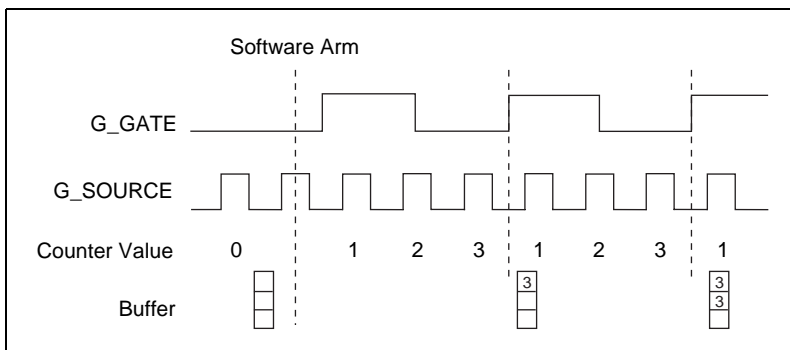
Figure 3-18. Buffered Periodic Event Counting
