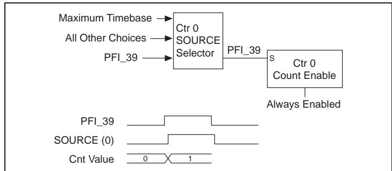
Figure 3-35. Without Synchronous Counting Mode
