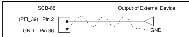
Figure 4-8. Wiring to Minimize Inductive Effects
