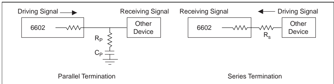
Figure 4-6. Parallel and Series Termination
