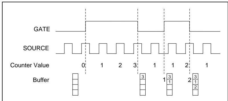
Figure 3-14. Buffered Semiperiod Measurement
