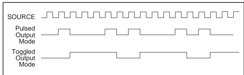
Figure 3-6. Output Modes
